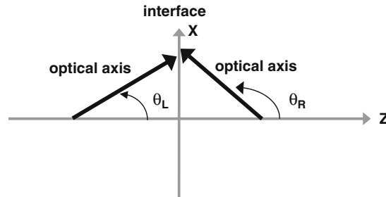
Fig. 1.2. The interface (the x - z plane) of two uniaxial anisotropic media
