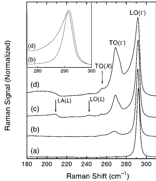
FIG. 1. (a) Raman spectrum of GaAs for 2.41-eV excitation; Raman spectra of the 1% N sample for various excitation energies: (b) off resonance, 2.41 eV, (c) near the E_+ resonance, 1.84 eV, and (d) near E_w , 1.76 eV. The arrows indicate two new phonon modes that become activated near resonance with E_+ . The inset compares the line shapes of the \text{LO}(\Gamma) line in spectra (b) and (d).
