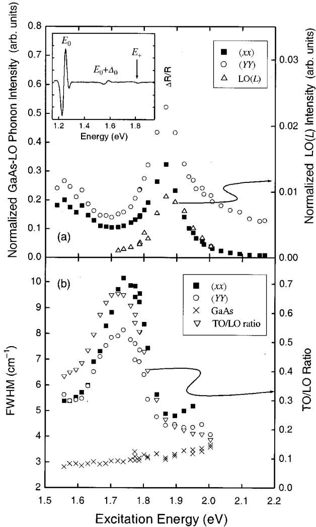
FIG. 2. (a) The intensity of the GaAs-like LO phonon lie of the 1% N sample as a function of the excitation energy for the allowed ( \circ ) and the forbidden ( \blacksquare ) polarization. The inset is an ER spectrum of the same sample from Ref. 4. The open triangles are the intensities of the L -point LO phonon peak at \sim 240 \text{ cm}^{-1} . (b) the FWHM of the GaAs-like LO phonon line as a function of the excitation energy for the 1% N sample. The ratio of the forbidden TO phonon intensity to the intensity of the allowed GaAs-like LO is also plotted. The FWHM of a LO phonon peak of a GaAs epilayer is presented for comparison.
