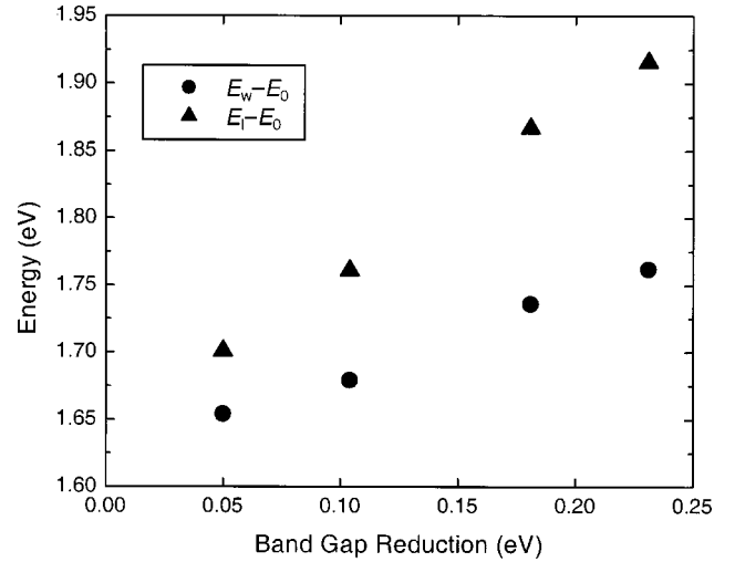
FIG. 3. E_I - E_0 and E_w - E_0 as functions of the band-gap reduction, \delta E_0 = E_0(\text{GaAs}) - E_0(\text{GaAs}_{1-x}\text{N}_x) .
