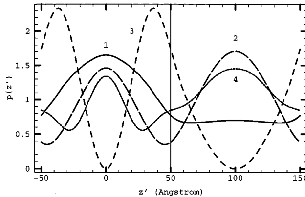
FIG. 3. Probability distributions of the first four band-edge states (labeled as 1–4) of symmetric OSL's with L_A = L_B = 100 \text{ \AA} : (a) type I and (b) type V.
