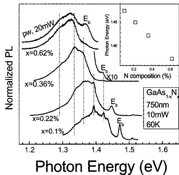
FIG. 2. The PL spectra of all four \text{GaAs}_{1-x}\text{N}_x ( x=0.1\% - 0.62\% ) samples at 60 K and under either cw or pw excitations. At the same time, the exact energy positions of the E_b emissions at 60 K are also shown in the inset.
