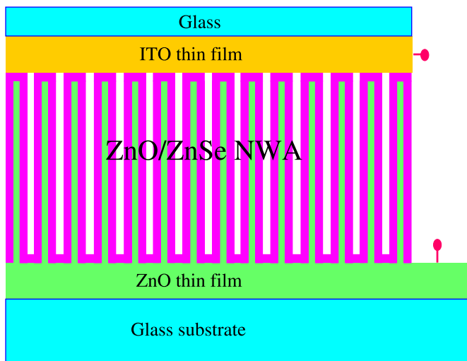
Fig. 1. Device structure.
