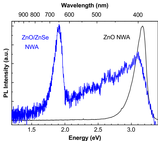
Fig. 3. Photoluminescence spectra (room temperature).
